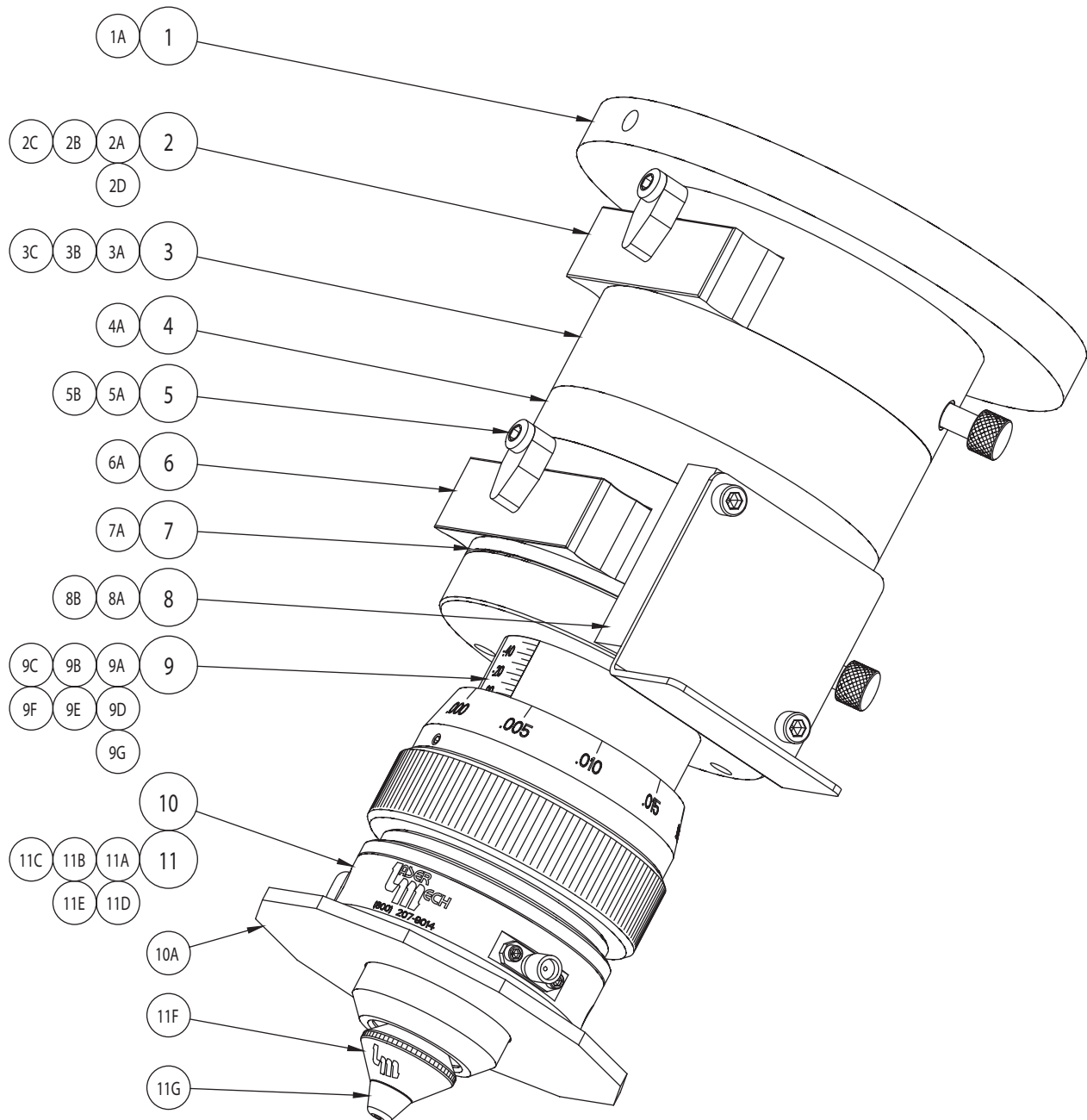
Alternate Tip Assembly (Saturn II)
